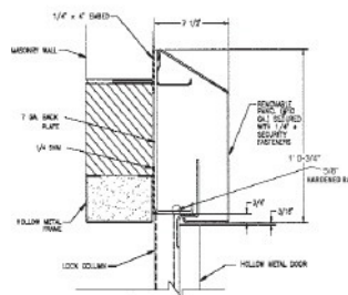
DETAIL A - SLOPED BOX
